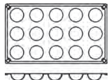
FR003 SEMISFERA Ø mm 40 x 20 H vol. 17 ml 15 impronte/indents
