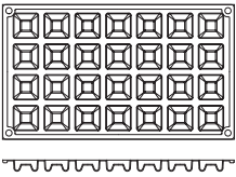
FR075 MICRO SAVARIN QUADRATO mm 30 x 30 x 13,5 H vol. 9,5 ml 28 impronte/indents
