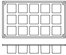
FR103 CUBO mm 40 x 40 x 40 H Vol. 62 ml 15 impronte/indents
